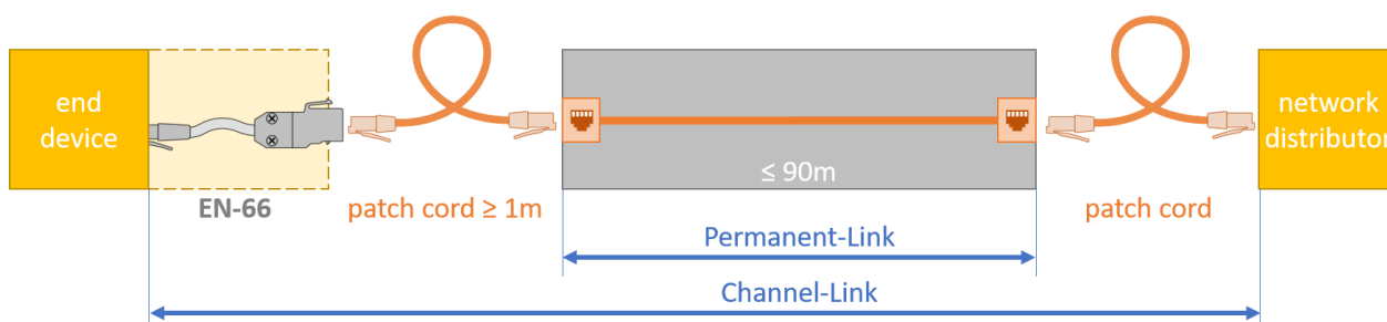
Figure 7 Recommended setup of the network isolator
