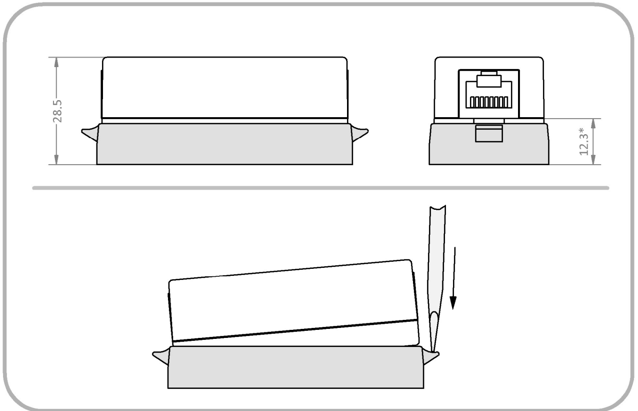
Mounting dimensions and unlocking of the Z6-W wall mounting plate All dimensions in mm Isolation distance between exposed metallic shield contacts and the mounting surface
