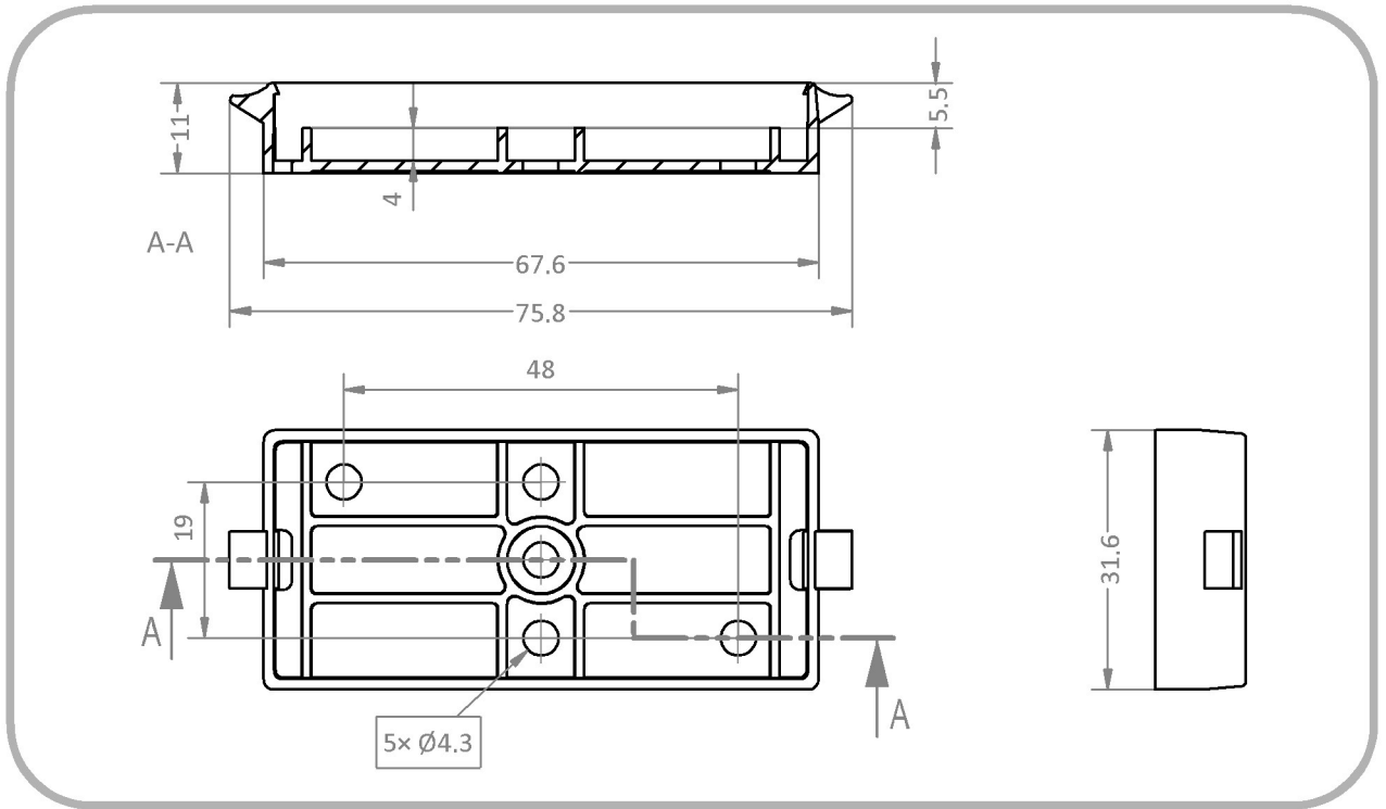
Dimensions of wall mounting plate Z-6W All dimensions in millimeters
