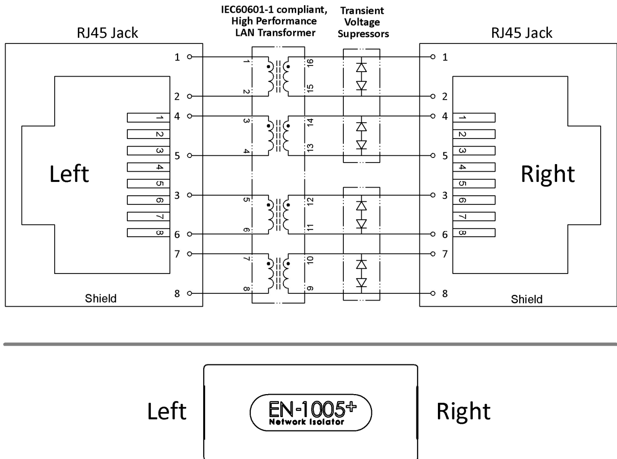
Figure 5. Schematic diagram of the EN-1005+.
