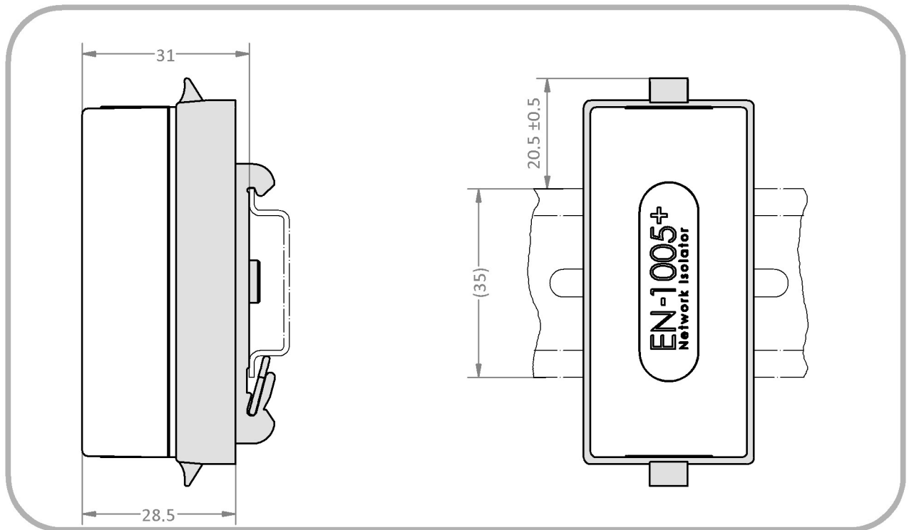
Assembly dimensions for the DIN rail adapter Z-6R with EN-1005+ All dimensions in millimeters
