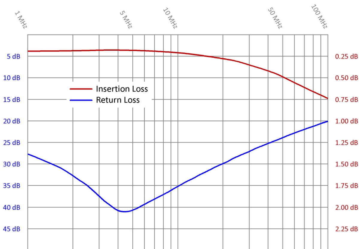
Figure 4. Typical frequency response for EN-1005*.
