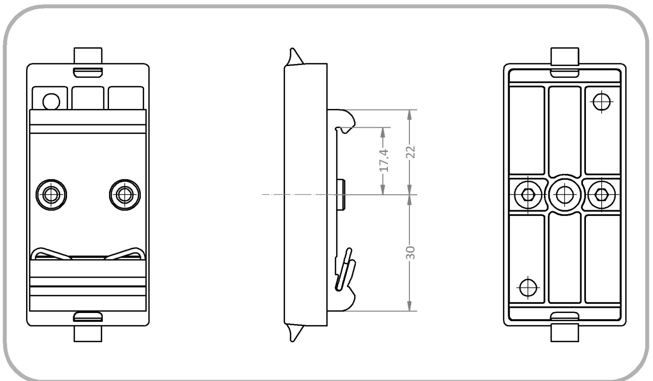
Dimensions of DIN rail adapter Z-6R All dimensions in millimeters
