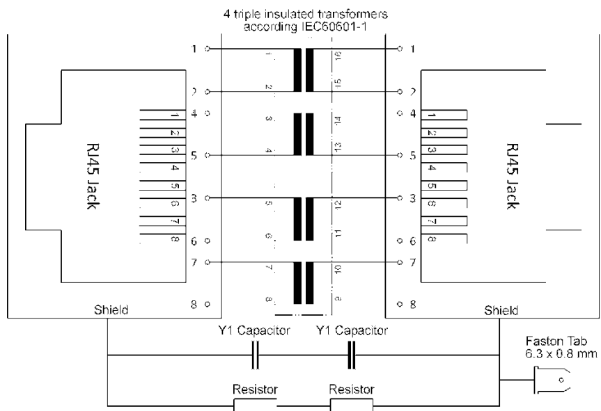
Figure 14. Circuit diagram for EN-50HG-S, EN-50VG-S, and EN-50HG-Y
